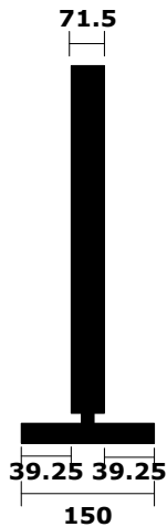
Side View (mm)
